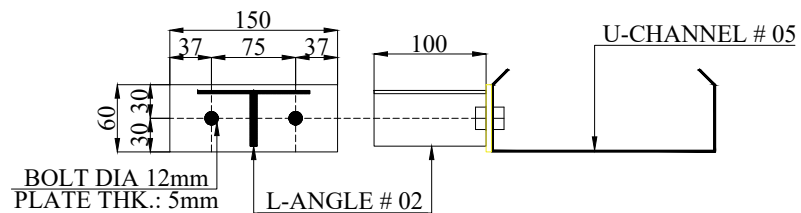
CONNECTION PLATE # 01
